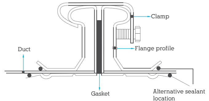
Typical cross section through the profile
